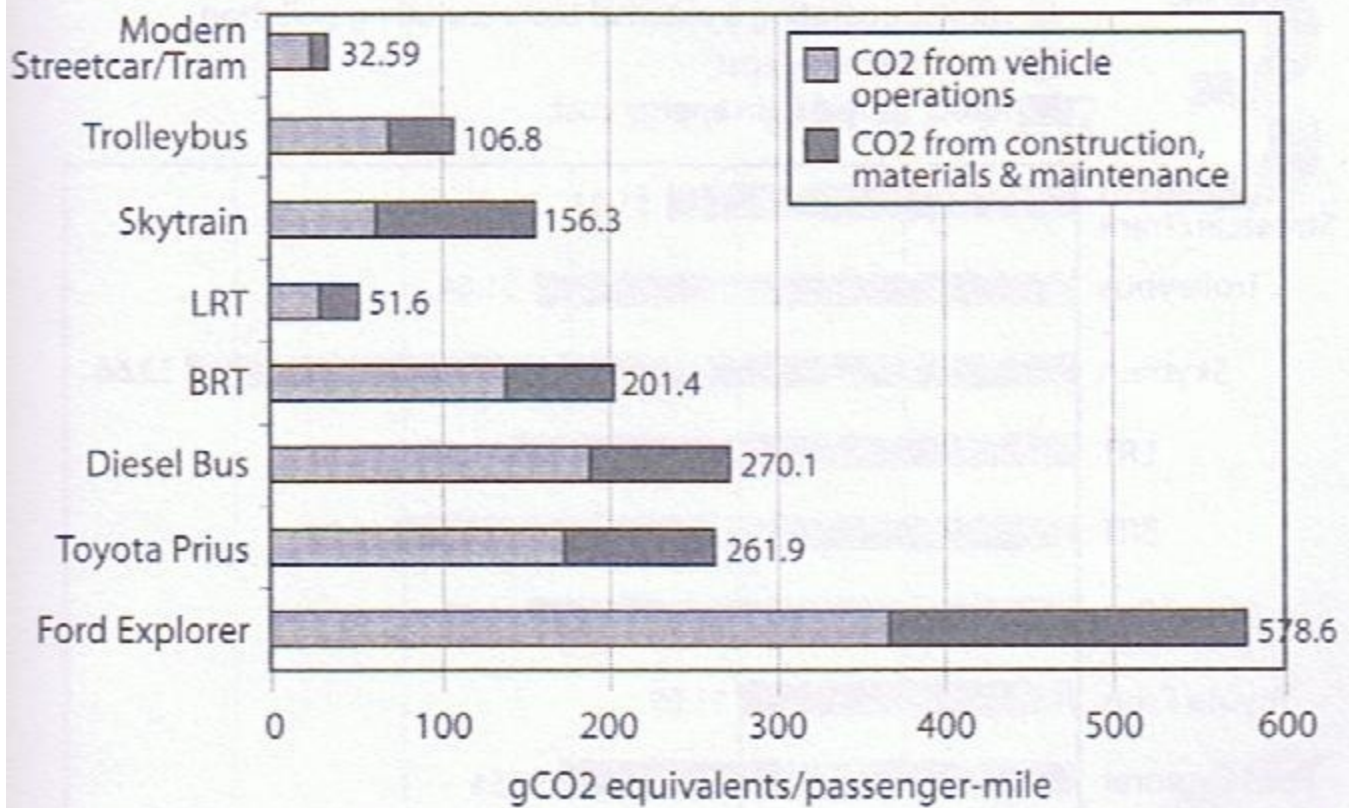
Figure 2.19. Carbon emissions per passenger-mile when electricity source is coal. (Source: Strickland, 2008; U.S. Environmental Protection Agency, 2005; Spadaro, Langlois, and Hamilton, 2000)
